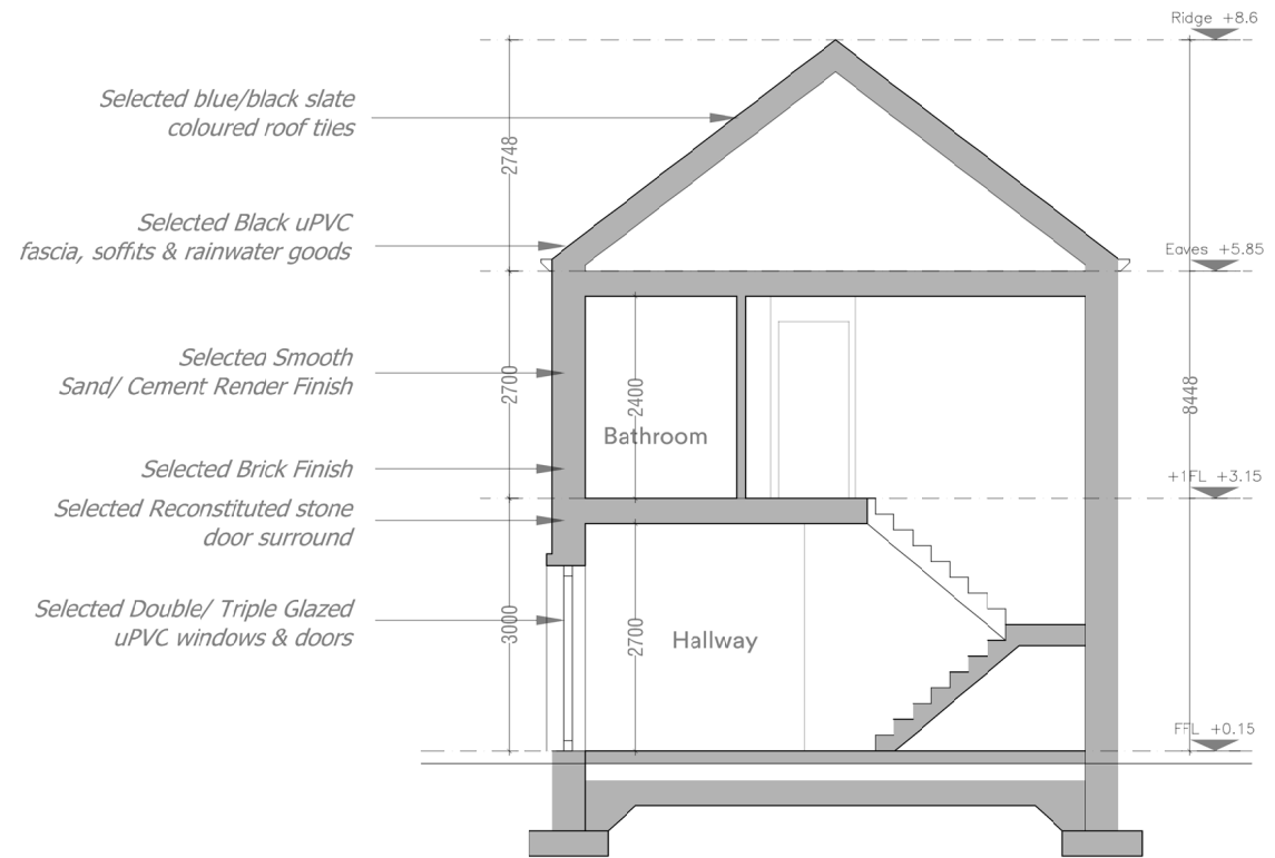
House Type U Detached Section A.A
