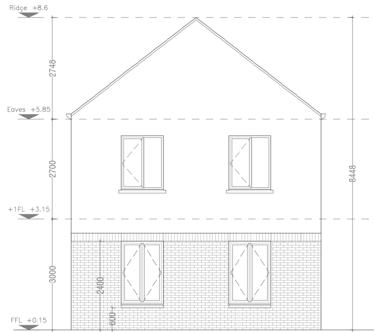
House Type U2 Semi - Detached Side Elevation
